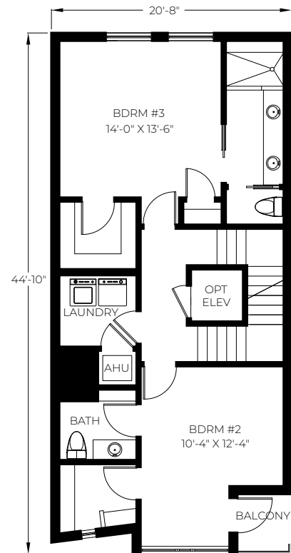
LVL 2-786 SF (LIVABLE)
