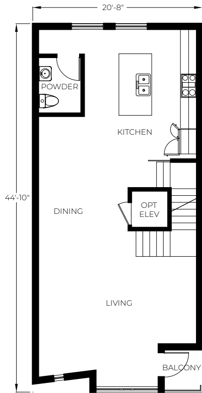
LVL 3-786 SF (LIVABLE)
