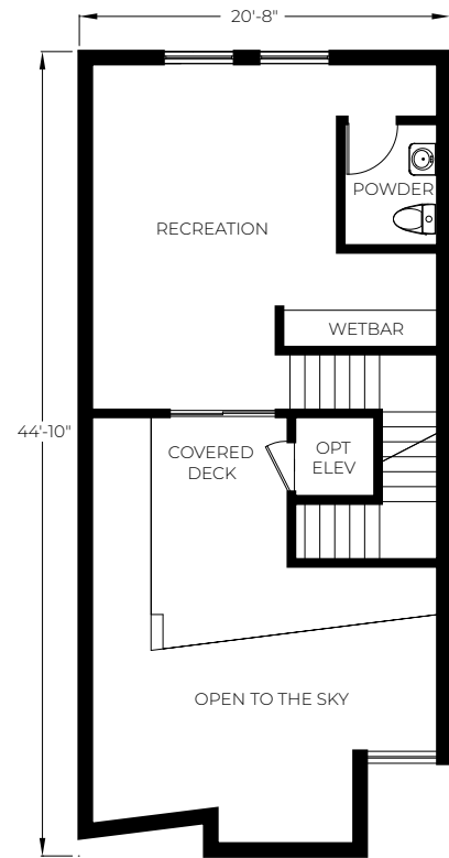
ROOF-OPTION - 441 SF
