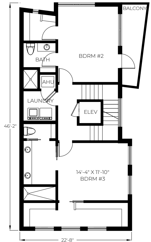
LVL 2 - 890 SF (LIVABLE)
