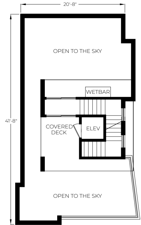
ROOF - STANDARD - 116 SF
